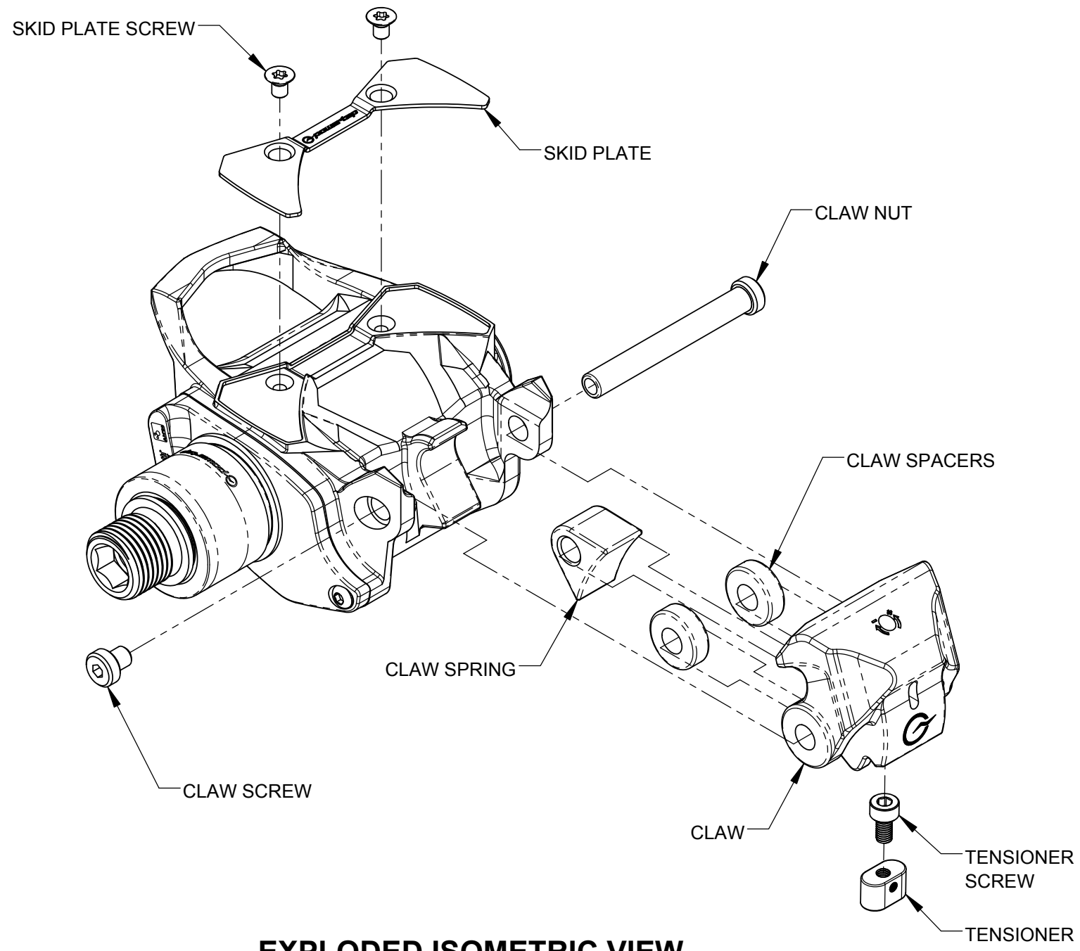
EXPLODED ISOMETRIC VIEW KIT,CLAW/SKID PLT REPLACEMENT (24416)
